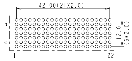
LAY-OUT P.C.B. - HOLE (FRONT SIDE)
